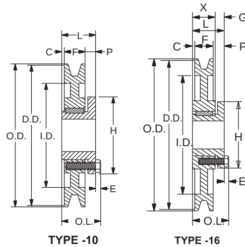
BUSHING DIMENSIONS
