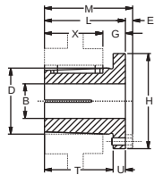
BUSHING
