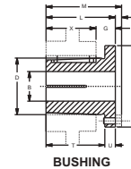
BUSHING
