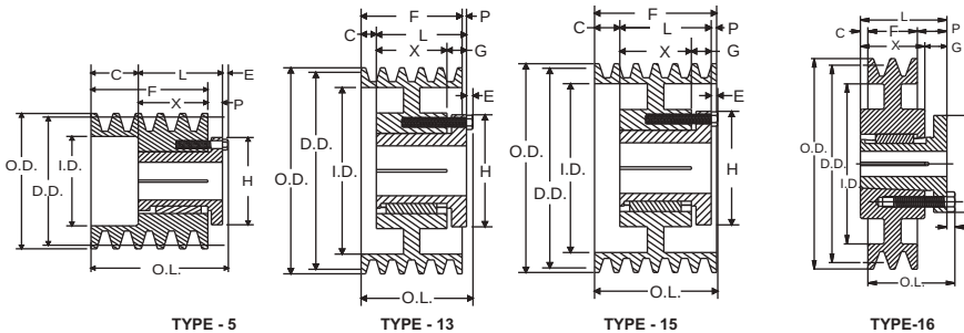
BUSHING DIMENSIONS
