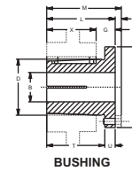
BUSHING
