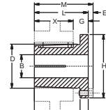
BUSHING
