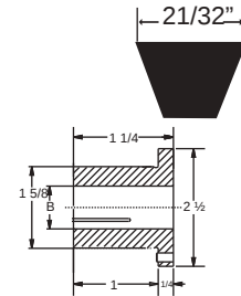
BUSHING
