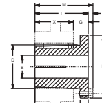
BUSHING
