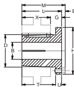
BUSHING
