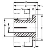
BUSHING
